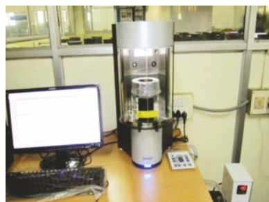
Process Tensiometer
